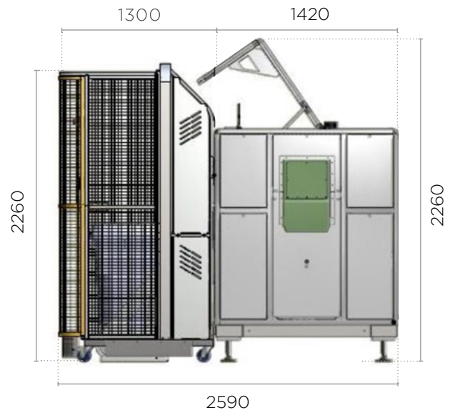
Side View Hatch fully opened
