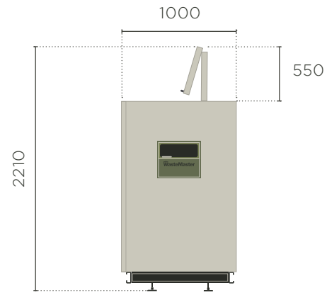
Side View Hatch fully opened
