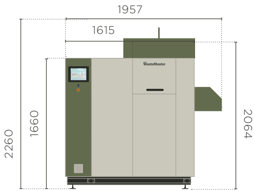
Front View Hatch fully opened
