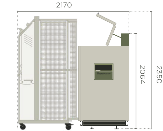
Side View Hatch fully opened
