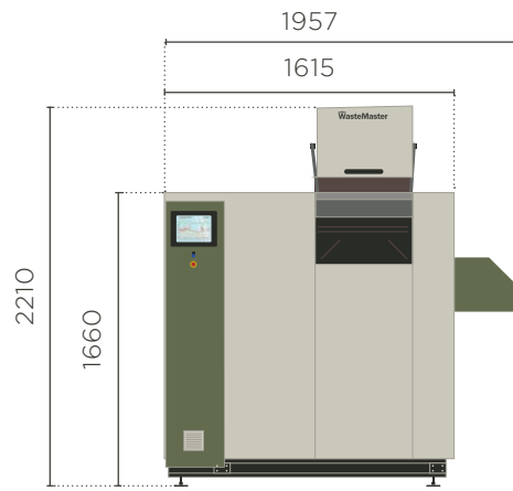
Front View Hatch fully opened and bin lifter presented
